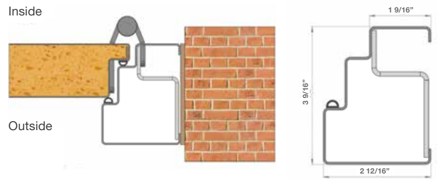
MITRED FRAME, OPEN TO INSIDE ( LI )
