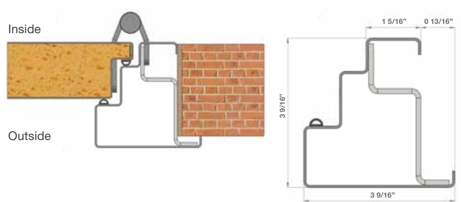
MITRED FRAME WITH MOULDINGS, OPEN TO INSIDE ( MI )
