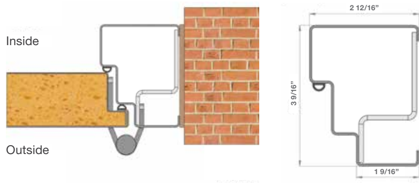
MITRED FRAME, OPEN TO OUTSIDE ( LO )
