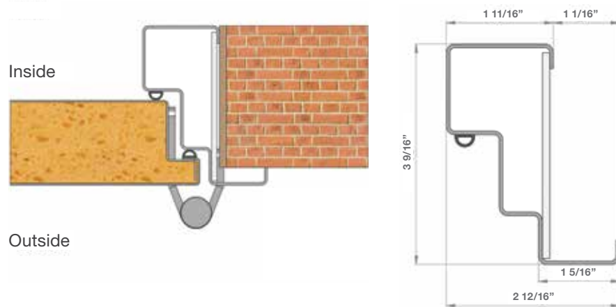
MITRED FRAME WITH MOULDINGS, OPEN TO OUTSIDE ( MO )
